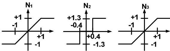
Fig.12. Nonlinearities of Example 3.
