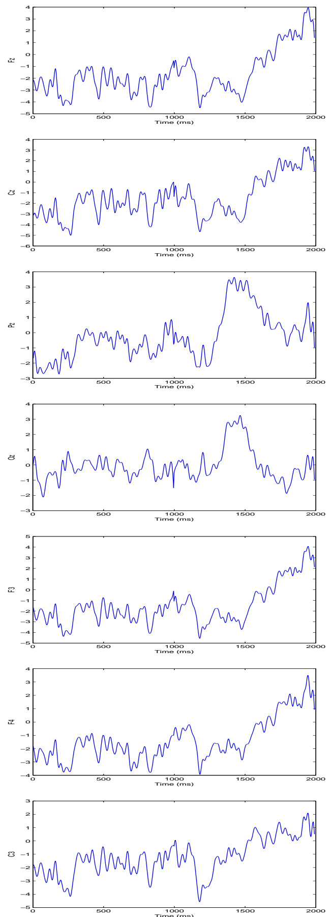
Fig. 1: ERP filtered data after artifact removing for 2 epochs, channels 1-7
