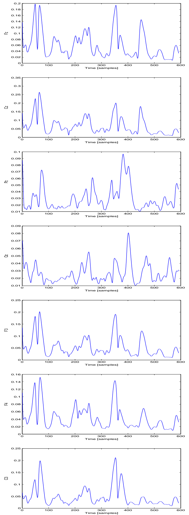
Fig. 5: Normalized Rényi information for ERP filtered data without artifacts: channels 1-7 (2 epochs)
