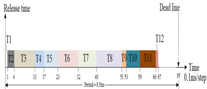
Figure 2. Tasks scheduling based on RM.
