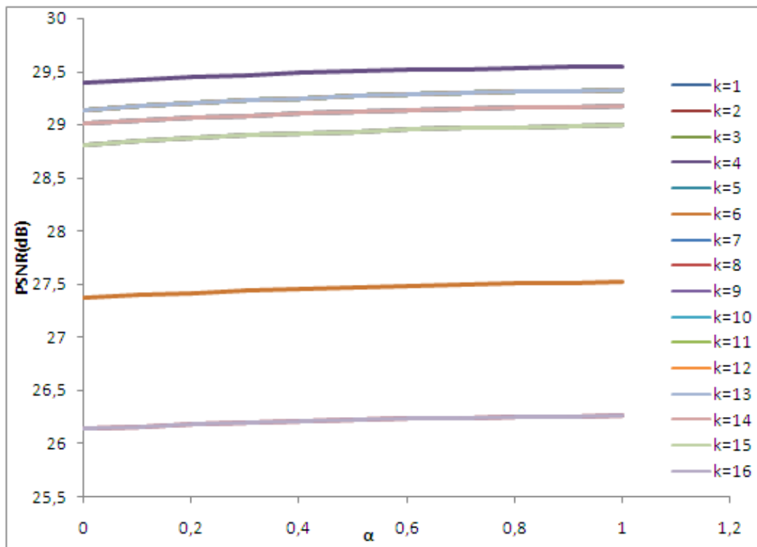
Figure 5: Selection of parameter k and the laplacian filter shape \alpha .
