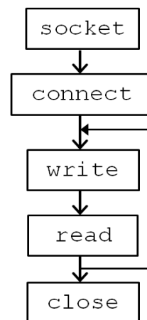
Fig 2 The basic algorithm for communications between a client and server
