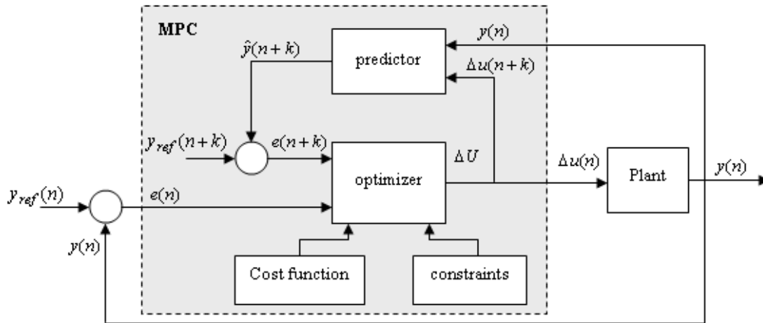
Fig. (2): Basic structure of model predictive control
