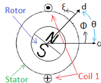
Fig. 4: Brushless Reference systems
