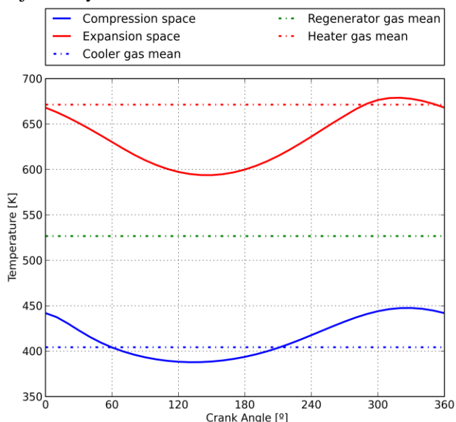
Fig. 8 Temperature variation in the heat exchangers, expansion and compression spaces, for a p_{mean} = 30 bar.
