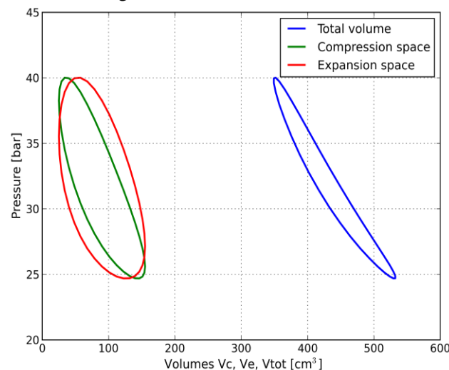
Fig.7 Pressure versus space volume diagrams for a p_{mean} = 30 bar.
