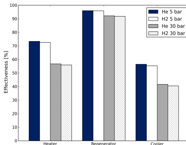
Fig. 10 Effectiveness results considering helium and hydrogen as working fluids at different values of mean pressure.
