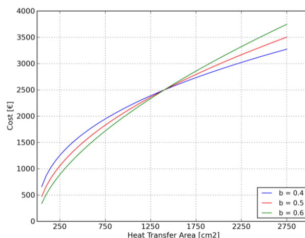
Fig. 5 Cooler cost estimation.
