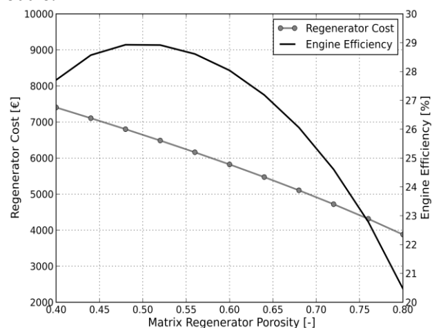
Fig. 13 Stirling engine efficiency and regenerator cost as a function of porosity of the regenerator matrix.
