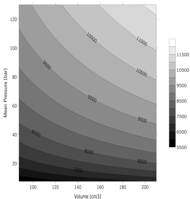
Fig. 6 Engine bulk cost estimation.
