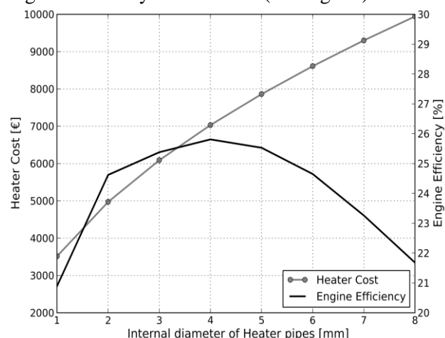
Fig. 12 Stirling engine efficiency and heater cost as a function of the internal diameter of the heater pipes.
