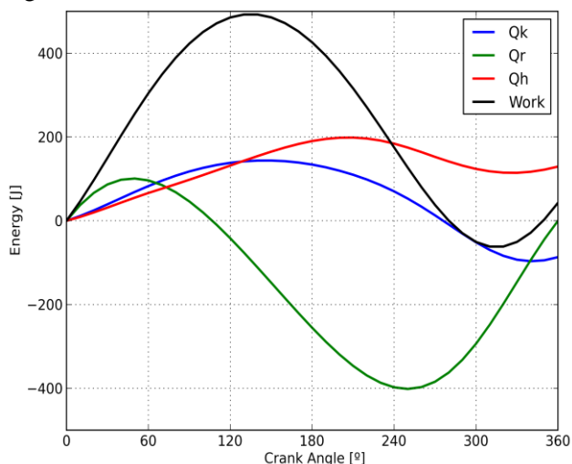
Fig. 9 Energy variation diagram for a p_{mean} = 30 bar.
