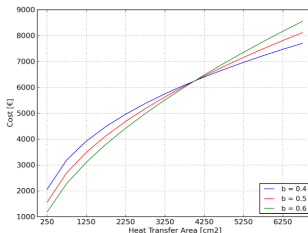
Fig. 4 Regenerator cost estimation.
