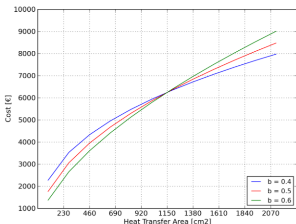
Fig. 3 Heater cost estimation.
