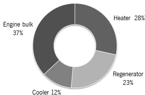
Fig. 11 Relative cost of each component of the Stirling engine.
