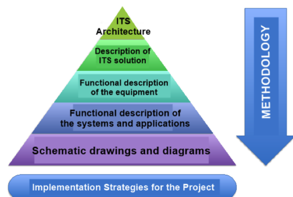
Fig.1: Development Methodology
