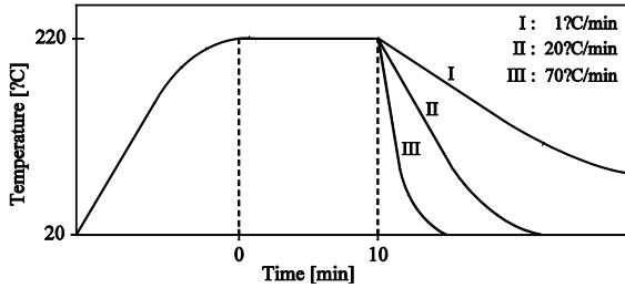
Fig.1. Schematic representation of the different thermal conditions applied during processing of commingled CF/PA12 composites.
