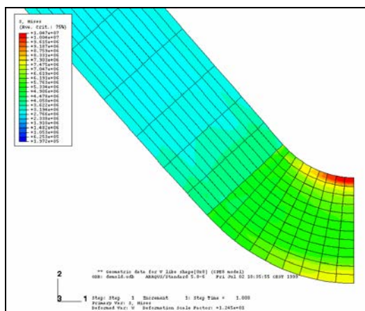
Fig.4 Von-Mises stresses of [90_8] , geometry of half a section of a U-shaped laminate after demoulding
