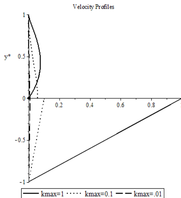
Fig. 3 Velocity Profiles u^*(y), v^*(y) , for \mathcal{G} = 1 and different values of k^*_{max} .
