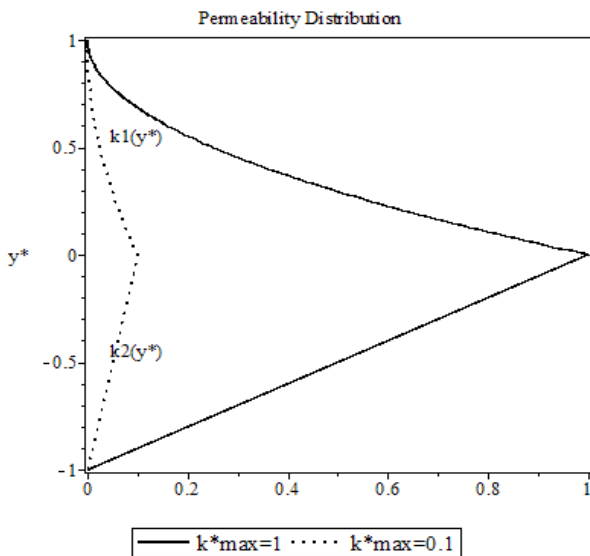
Fig. 2. Permeability Distribution in the Two Layers
