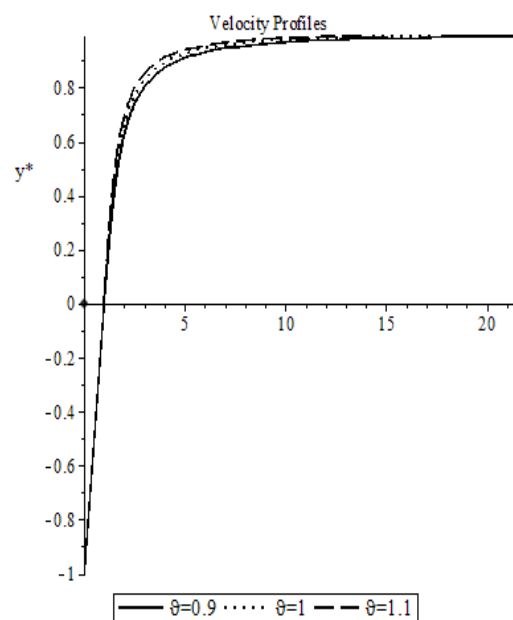
Fig. 4 Velocity Profiles u^*(y), v^*(y) , for k^*_{max} = 1 , and different values of \mathcal{G} .
