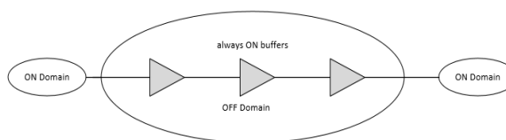
Fig 6 AON buffers placed in OFF domain to allow communication between two ON domains
