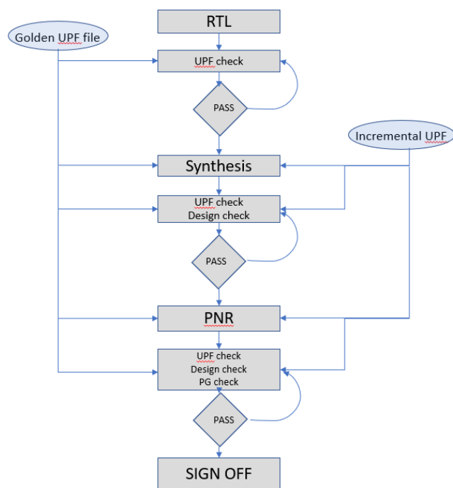
Fig 9 VCLP design flow
