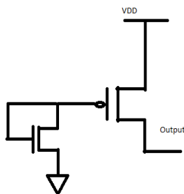
Fig 16 Tie high cell
