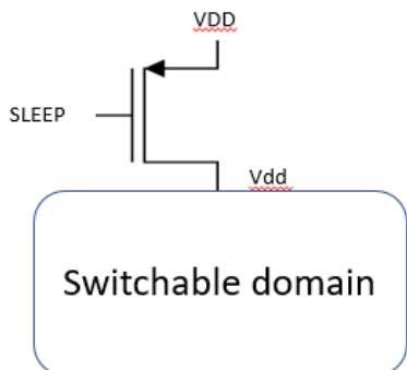
Fig 7 Header power switch
