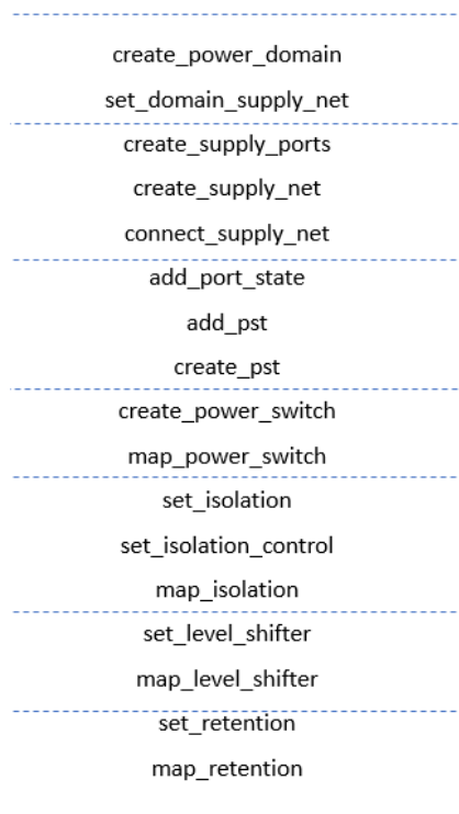
Fig 8 UPF file structure
