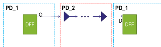
Fig 18 Adding setup/hold buffers
