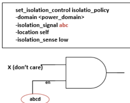
Fig 11 The isolation signal mentioned in the UPF is different from the design
