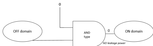
Fig 2 Signal transmission with isolation cell
