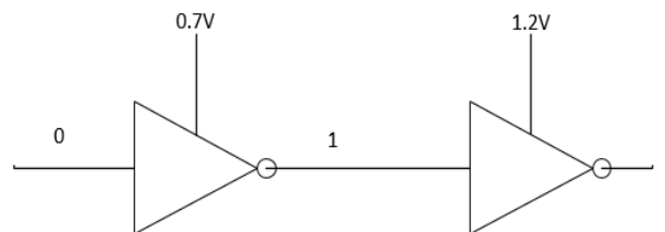
Fig 4 Showing need of LS from low to high voltage levels
