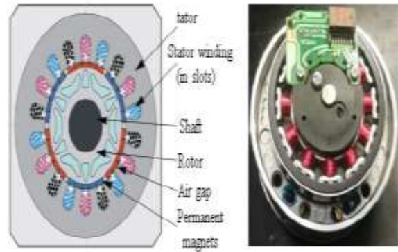
Figure (9). Basic BLDC motor construction [17]
