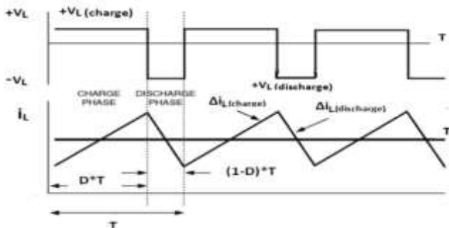
Figure (4) Waveforms of Buck-Boost converter
