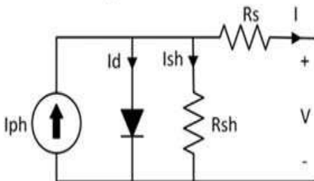
Figure (1) equivalent circuit of solar cell
