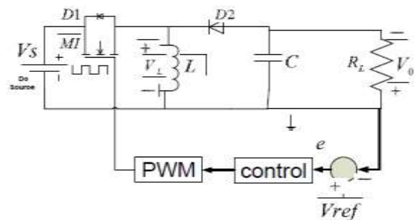
Figure (3) DC-DC Buck Boost Converter System used in simulations.
