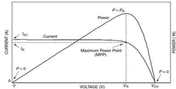
Fig. 2. characteristic curve of a PV module
