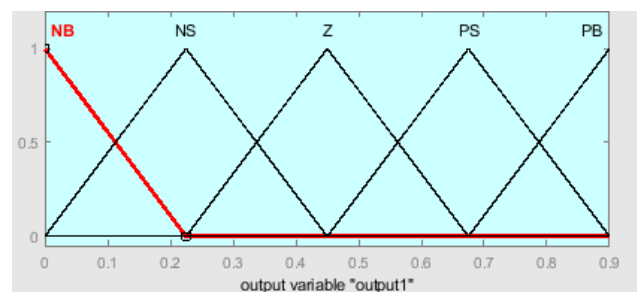
Fig (8) Membership function of duty cycle change.
