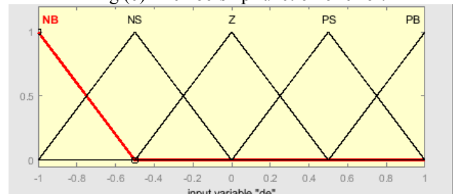
Fig (7) Membership function of error change..
