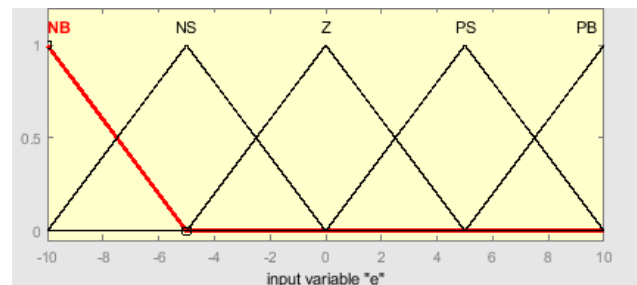
Fig (6) Membership function of error.
