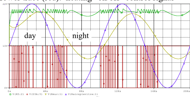
Figure 7: High amplitude outside air temperature variation
