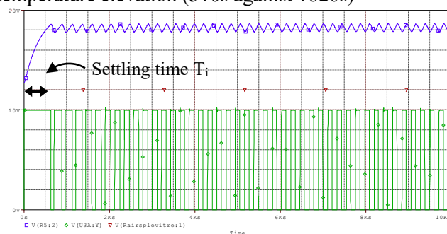
Figure 9: Transient and steady state response with internal insulation n^{\circ}2 (polystyrene)
