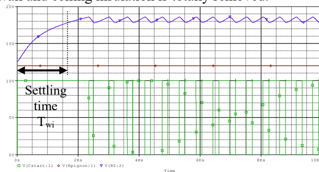
Figure 8: Transient and steady state without internal insulation
