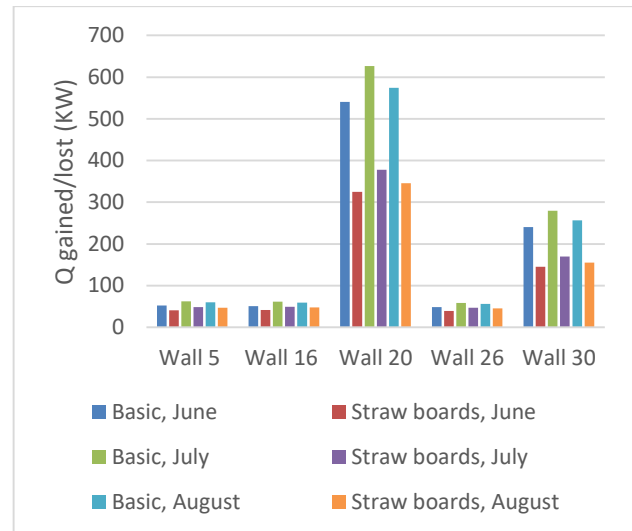
Fig 9: Basic vs Straw Boards heat gained through walls
