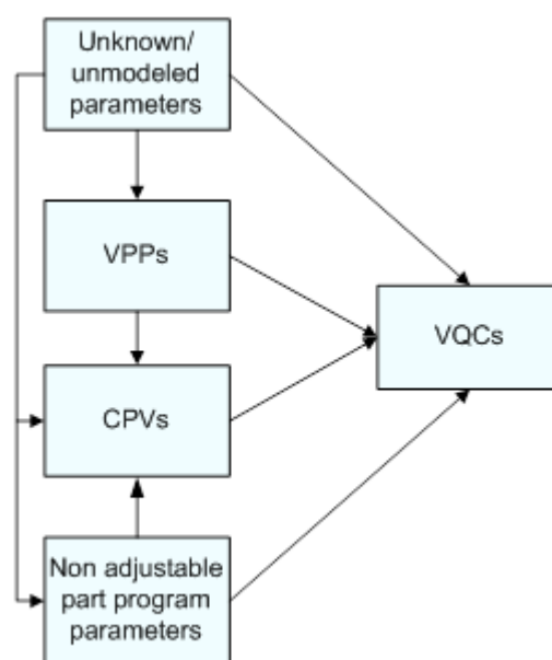
Fig. 1: Links between the types of parameters involved in part quality prediction.
