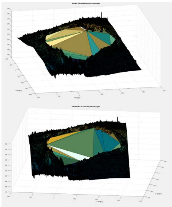
Fig. 10. Different Delaunay surfaces on the 3D model of active open pit mine
