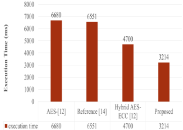
Fig.10 Comparison of the execution time of the algorithm with other studies [12-14]
