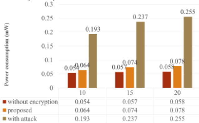
Fig.7 Power Consumption (mW)
