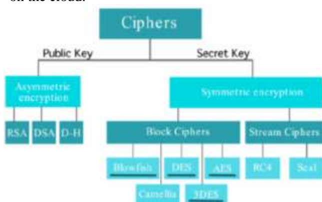
Fig.1 Classification of cryptographic algorithms [6]
