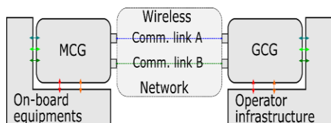
Fig. 1. Scheme of communication between train and ground infrastructure.
