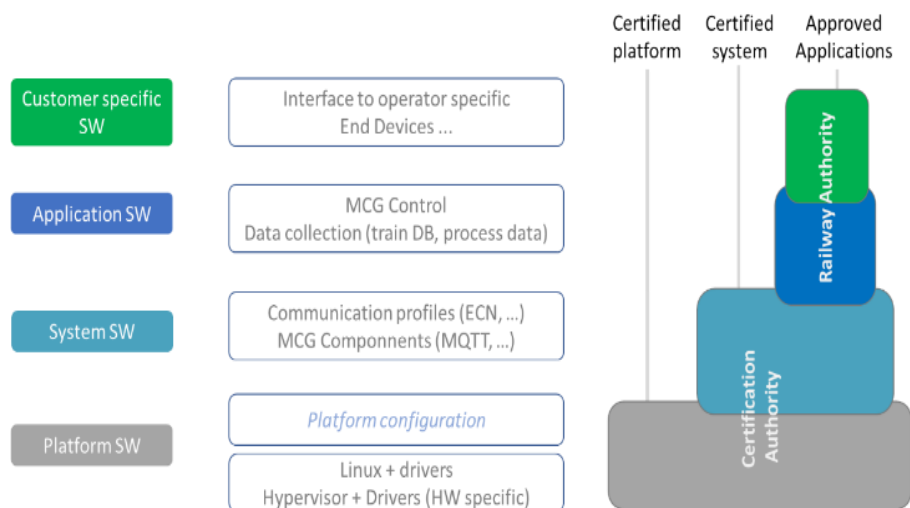
Fig. 3. MCG software structure.
