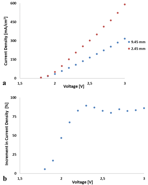
Fig. 6. a) Polarization curves at 9.45 and 2.45 mm of distances between electrodes and b) percentage of increment in current density between these distances.
