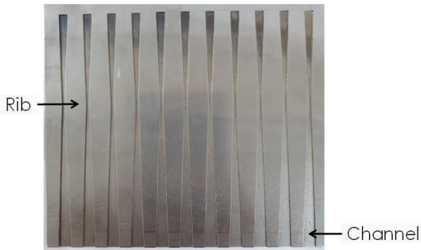
Fig 1. The electrode with the triangle shaped topology.
