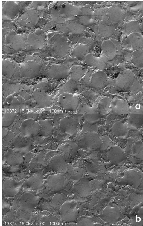
Fig. 2. SEM micrographs of surface channel zones in CH33 electrode: a) rougher 100 x and b) smoother 100 x.
