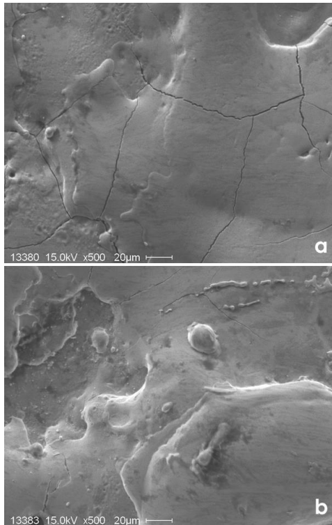
Fig. 9. SEM micrographs of two electrodes with different surface roughness: a) 4.5 µm Ra (500 x); b) 12.6 µm Ra (500 x) [14].
