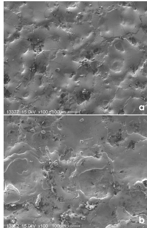
Fig. 8. SEM micrographs of two electrodes with different surface roughness: a) 4.5 \mu\text{m Ra} (100 x); b) 12.6 \mu\text{m Ra} (100 x) [14].
