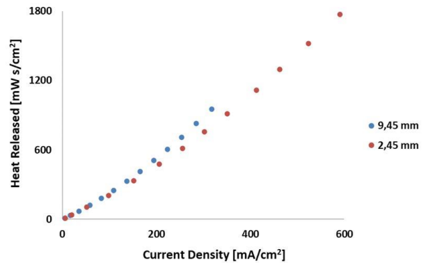
Fig. 7. Heat released as a function of current density for the 9.45 and 2.45 systems.
