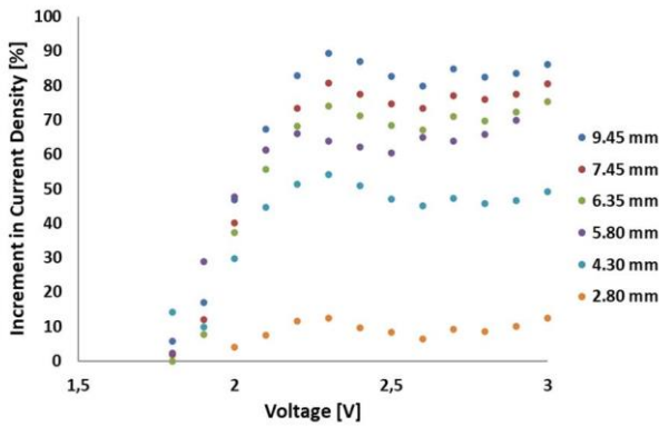
Fig. 4. Percentage of increase in current density with respect to the closest distance evaluated: 2.45 mm
