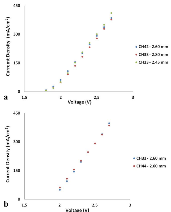
Fig. 10. Polarization curves at different distances between electrodes.
