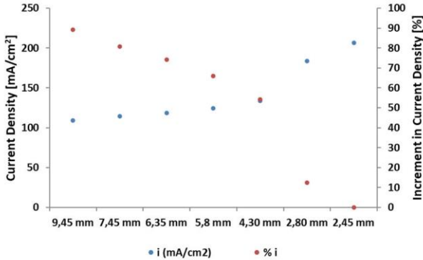
Fig. 5. Current density and percentage of increment for an applied voltage difference of 2.3 V.
