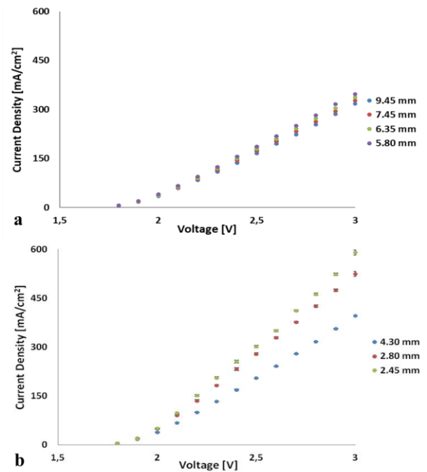
Fig. 3. Polarization curves per unit area for the analyzed distances between electrodes: (a) 9.45; 7.45; 6.35 and 5.80, and (b) 4.30; 2.80 and 2.45 millimeters.
