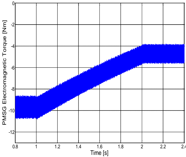
Fig. 8 The PMSG electromagnetic torque
