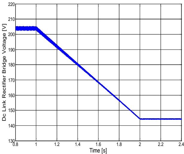
Fig. 9 The dc link rectifier bridge voltage
