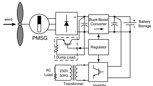
Fig.1 Wind turbine system configuration
