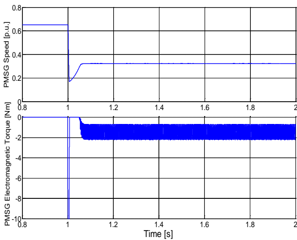
Fig. 4 PMSG rotor speed and electromagnetic torque
