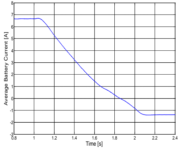
Fig.10 The battery average current
