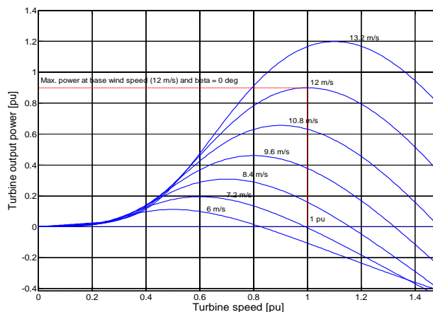
Fig. 3 Wind turbine characteristics at 3 kW
