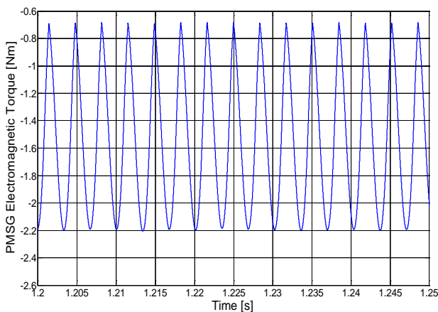
Fig. 5 PMSG electromagnetic torque variation
