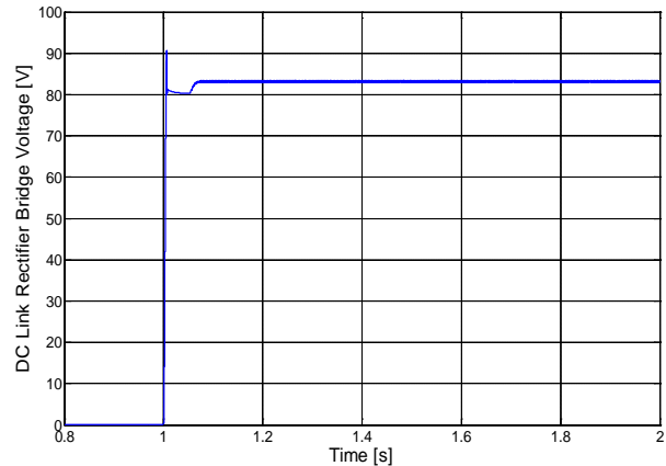
Fig. 6 The dc link rectifier bridge voltage
