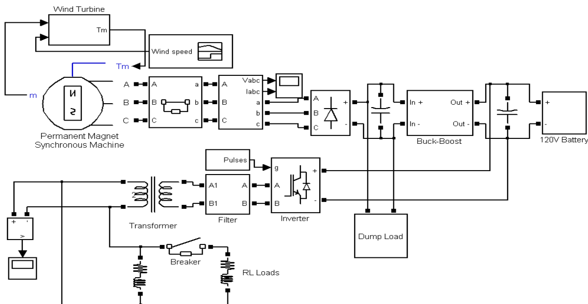
Fig. 2 Simulink diagram of the wind system
