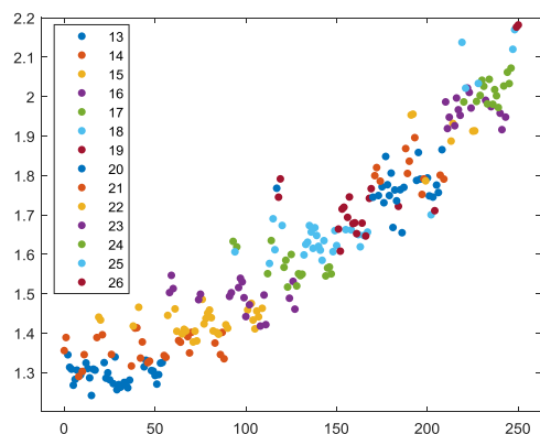
Figure 11: Relationship between the vibration amplitude (mm/s) and pressure across the turbine (daPa) grouped by power output (kW)
