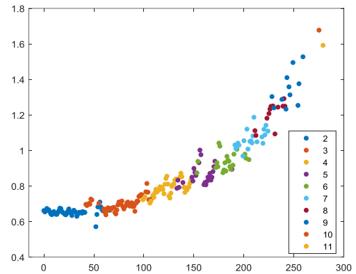
Figure 5: Relationship between the vibration amplitude (mm/s) and the pressure across the turbine (daPa) grouped by power output (kW)
