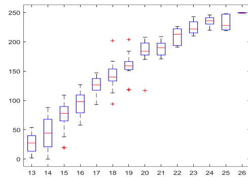
Figure 10: Relationship between the power output (kW) and the amplitude of the vibration (mm/s)
