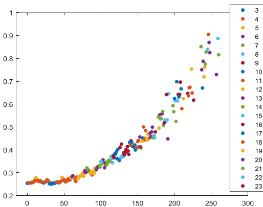
Figure 8: Relationship between the vibration amplitude (mm/s) and the pressure across the turbine (daPa) grouped by power output (kW)
