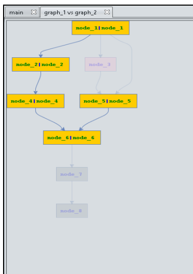
Fig. 8. The tab with the result of comparing the two graphs.
