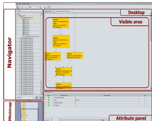
Fig. 2. Screenshot of user interface of the Visual Graph system.
