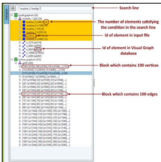
Fig. 3. Screenshot of the filter instrument.
