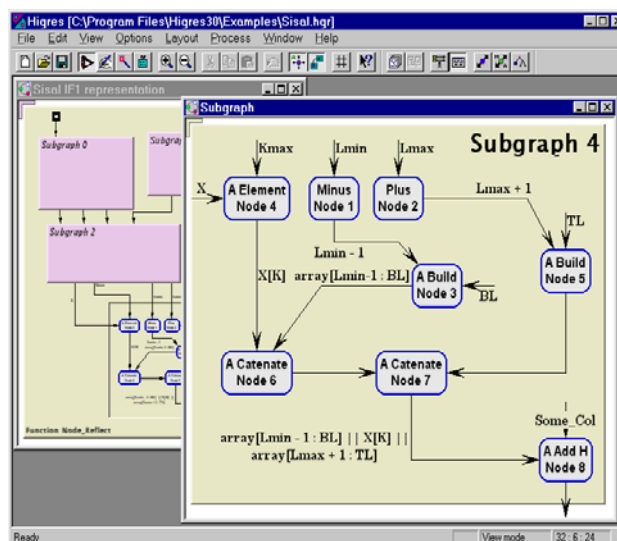
Fig. 15. Screenshot of the Higras system.
