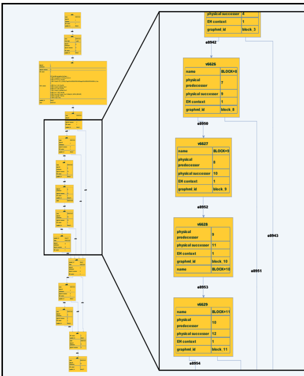
Fig. 11. Screenshot of using the hierarchical layout for control flow graph.
