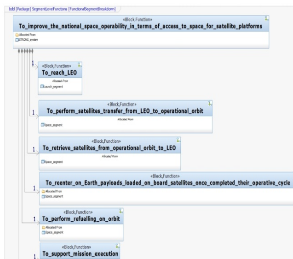
Figure 5: BDD for segment functional breakdown of STRONG system
