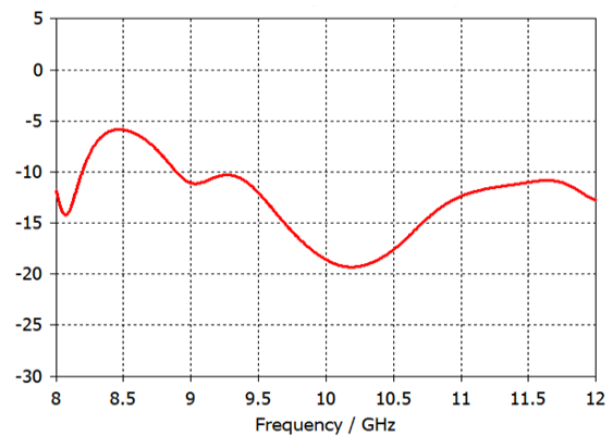
Fig. 4 Return loss.
