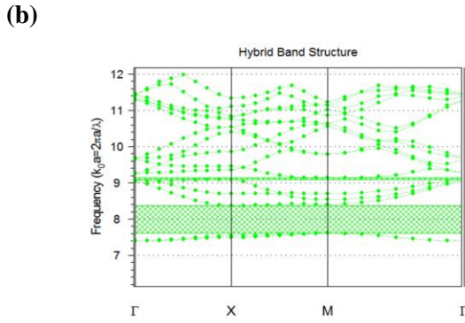
Figure 9. Band structures for the silica/air square lattice (a) for \beta=0 and (b) for \beta = 2.25 \mu m^{-1}
