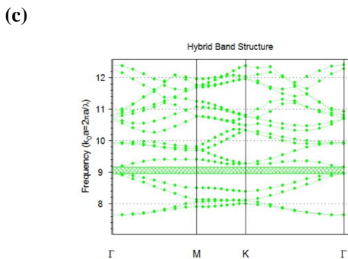
Figure 14. (a) Photonic crystal fiber with silica/air hexagonal air holes arrays and filling the third ring by silicon, (b) band diagram for \beta = 0 , and (c) for \beta = 9/\lambda .
