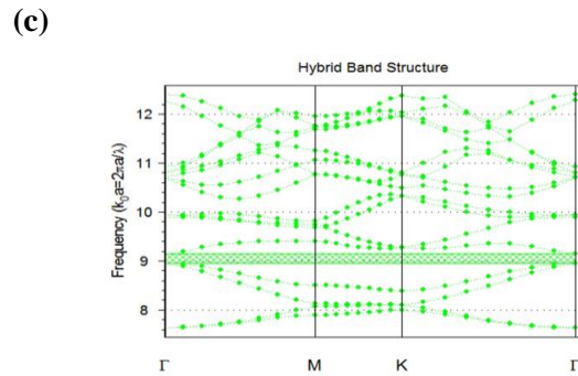
Figure 15. (a) Photonic crystal fiber with silica/air hexagonal air holes arrays and filling the fourth ring by silicon, (b) band diagram for \beta = 0 , and (c) for \beta = 9/\lambda .
