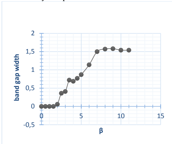
Figure 2. Variation of the band width for the silica/air hexagonal lattice versus the propagation constant \beta(\mu m^{-1}) .
