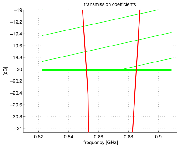
Figure 6: Detailed transmission coefficients of the optimized geometry of the FSS IEEE 802.11ah filter.
