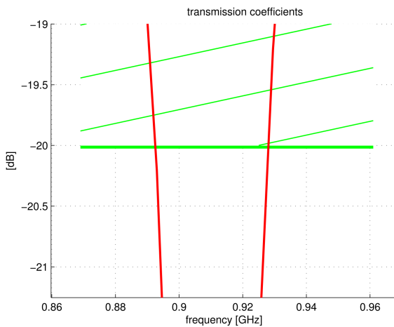
Figure 8: Detailed transmission coefficients of the optimized geometry of the FSS IEEE 802.11ah filter (US region).
