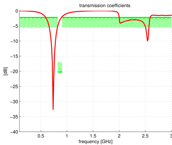
Figure 4: Transmission coefficients of the initial geometry of the FSS IEEE 802.11ah filter.
