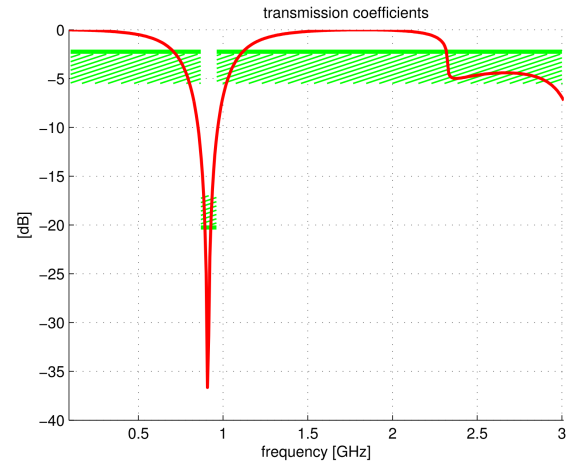
Figure 7: Transmission coefficients of the optimized geometry of the FSS IEEE 802.11ah filter (US region).
