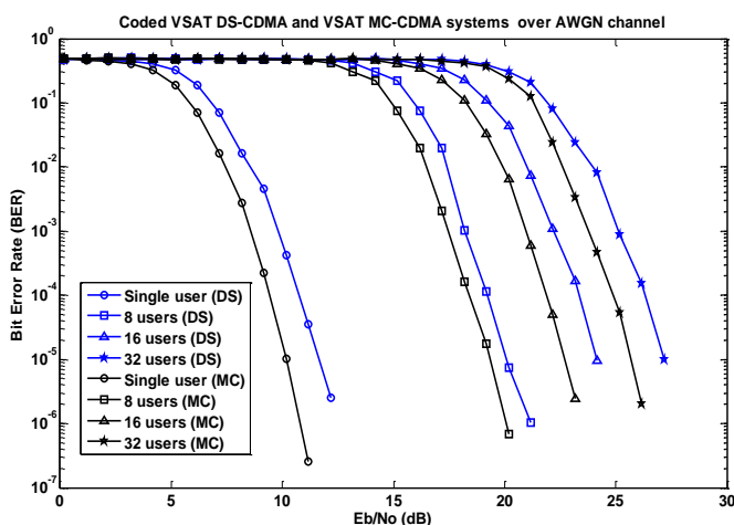
Fig. 10 Performance of coded VSAT DS-CDMA and VSAT MC-CDMA systems over AWGN channel
