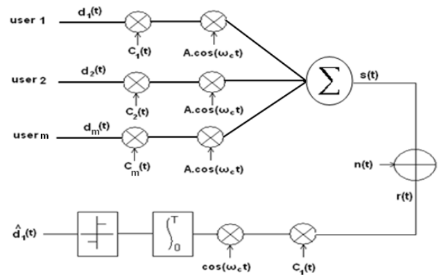
Fig. 3 Block diagram of DS-CDMA system transmitting over a Gaussian channel
