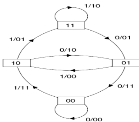
Fig. 7 The state-transition diagram for the encoder in Fig. 6
