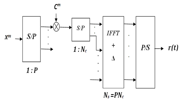
Fig. 4 MC-CDMA Transmitter
