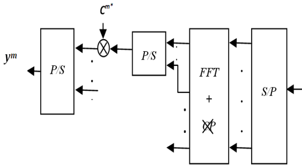
Fig. 5 MC-CDMA Receiver
