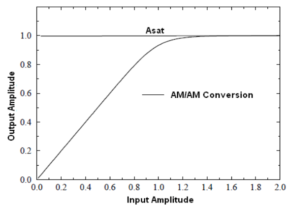
Fig.8 The SSPA characteristics : Normalized AM/AM conversion ( A_{sat}=1 )
