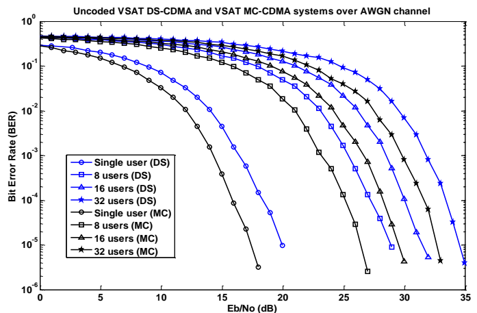
Fig. 9 Performance of uncoded VSAT DS-CDMA and VSAT MC-CDMA systems over AWGN channel
