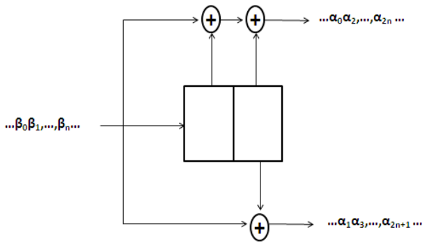
Fig. 6 A rate r = 1/2 memory m = 2 convolutional encoder
