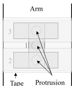
Fig0 17: Arrangement of three piezoelectric elements
