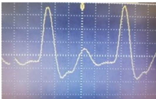
Fig0 7: An example of the extracted waveform obtained by inserting a protrusion (20 mV/div, 322ms/div), [11]
