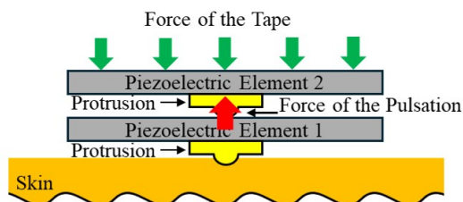
Fig0 14: Force applied to piezoelectric element 2 when two piezoelectric elements are stacked.
