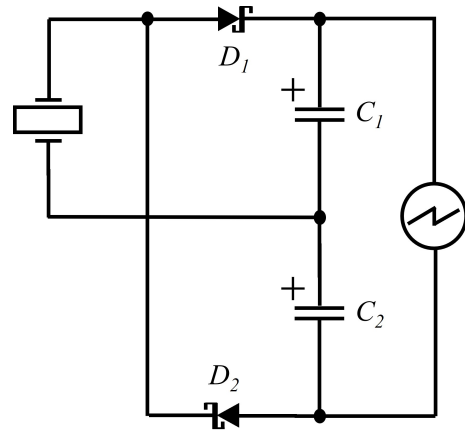
Fig. 24: Capacitor charging using a voltage-doubler rectifier circuit
