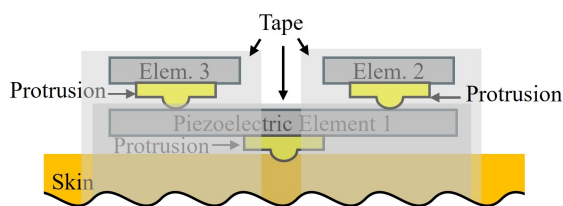
Fig018: Fixing arrangement of three piezoelectric elements
