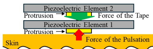
Fig0 35: Force applied to piezoelectric element 1 when two piezoelectric elements are stacked
