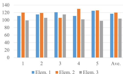
Fig019: "Maximum voltage of three piezoelectric elements
