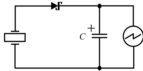
Fig. 23: Half-wave rectification circuit terminating in a single capacitor
