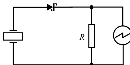
Fig0 20: "Half-wave rectification circuit using a Schottky barrier diode
