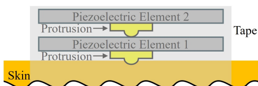
Fig0 11: Two piezoelectric elements on the skin viewed from the side
