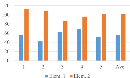
Fig0 12: Maximum voltage (mV) of two piezoelectric elements
