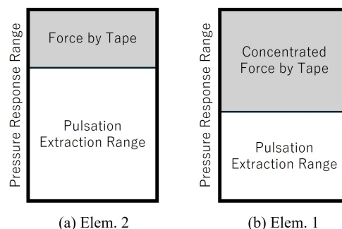
Fig0 16: Illustration of why the output voltage of Piezoelectric Element 1 reduces
