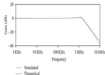
Figure.6. CMOS Simulated Gain and Phase Response of Low Pass Filter
