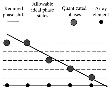
Fig. 3 Allowable phase state due to ideal quantization.
