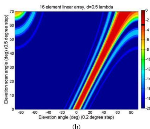
Fig. 2: (a) Overlapped simulations in a rectangular classical plot. (b) Unconventional color polar plot.
