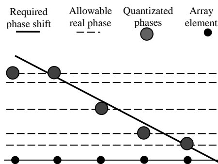
Fig. 4 Allowable phase state due to simulated real quantization.
