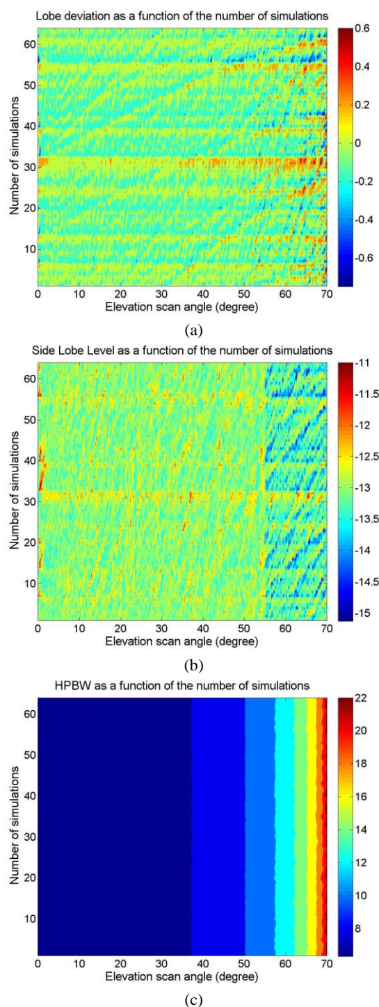
Fig. 8 Simulation results obtained changing the error phase vector. (a) Lobe deviation. (b) Side Lobe Level. (c) Half Power Beamwidth.
