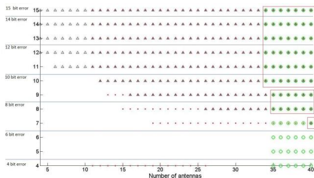
Fig. 6 Output results as function of bit-equivalent rms error for Lobe deviation < 0.005^\circ ; HPBW \le 3^\circ ; sll \ge -13\text{dB} . Compact view.
