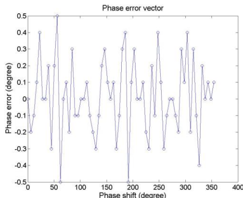
Fig. 7 Phase shifter error vector
