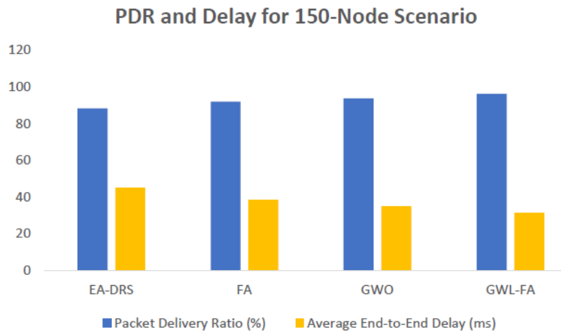
Figure 3: PDR and Delay for 150-Node Scenario
