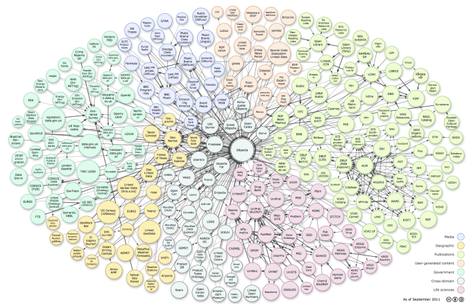
Fig. 1. Link Open data Cloud as of September 2011 (Cyganiak & Jentzsch)
