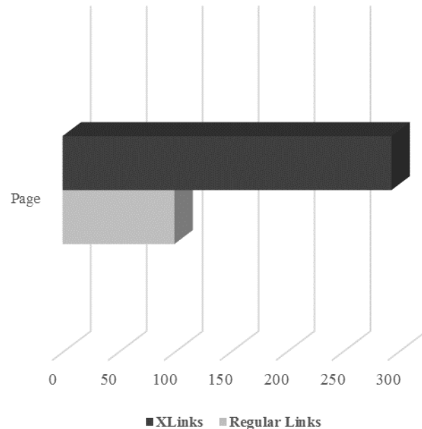
Fig. 5. Link Enrichment with XLink
