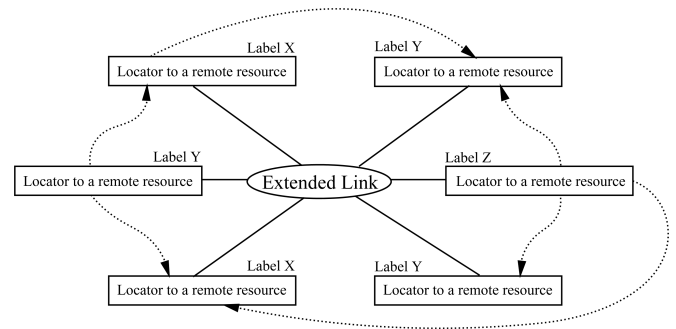
Fig. 2. Extended links with arc elements
