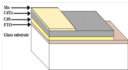
Figure : 1 The structure of the fabricated sensor.
