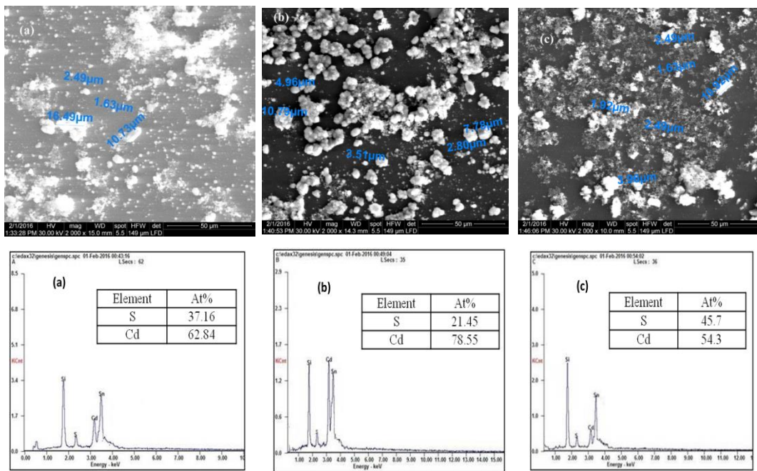
Figure : 2 SEM micrographs of CdS films deposited with different deposition times: (a)2hours, (b)3hours, (c)4hours.
